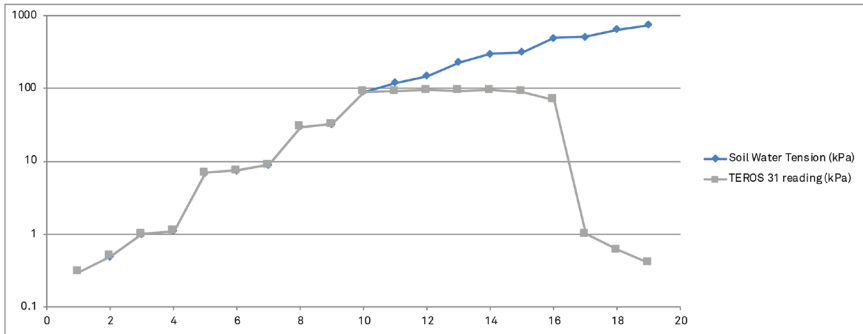
Figure 11 Tensiometer readings with tensions to -1,000 kPa
