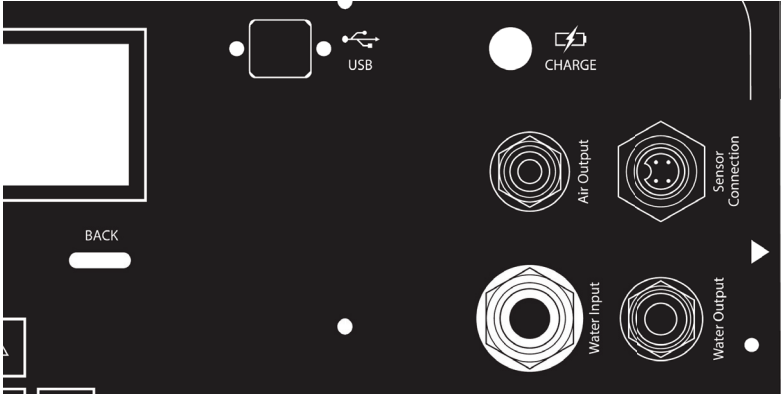
Figure 7 Charging port
