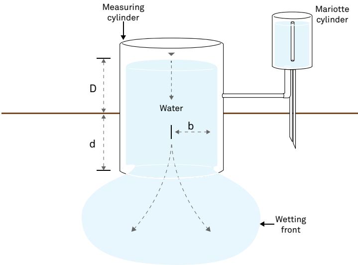
Figure 32 Cross section of a single-ring infiltrometer
