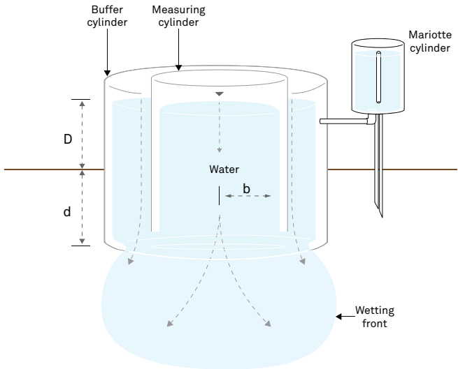
Figure 33 Cross section of a double-ring infiltrometer
