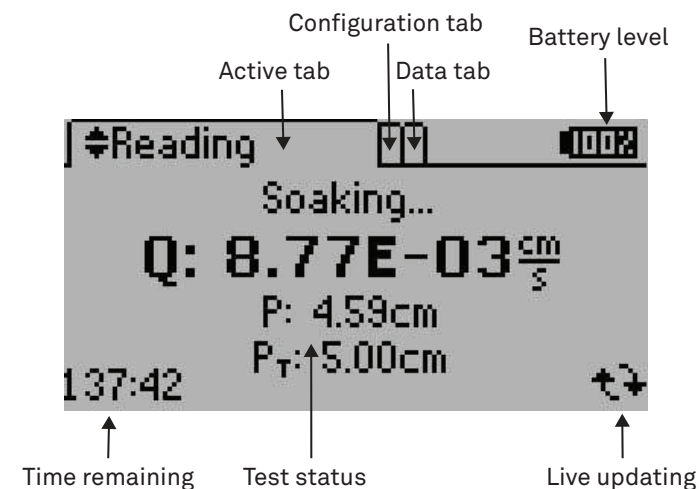
Figure 16 SATURO display elements
