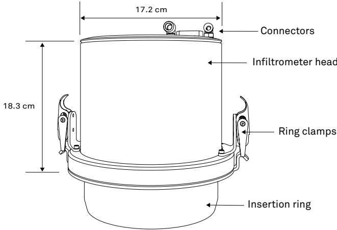
Figure 30 Infiltrator head
