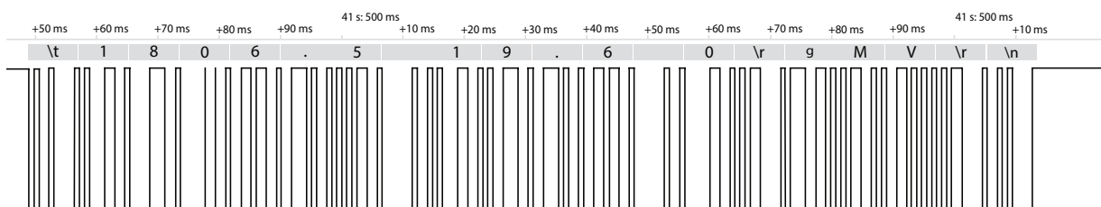
Figure 7 Example DDI Serial transmission
