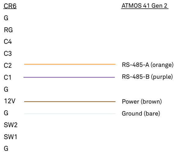
Figure 11 RS-485 interface
