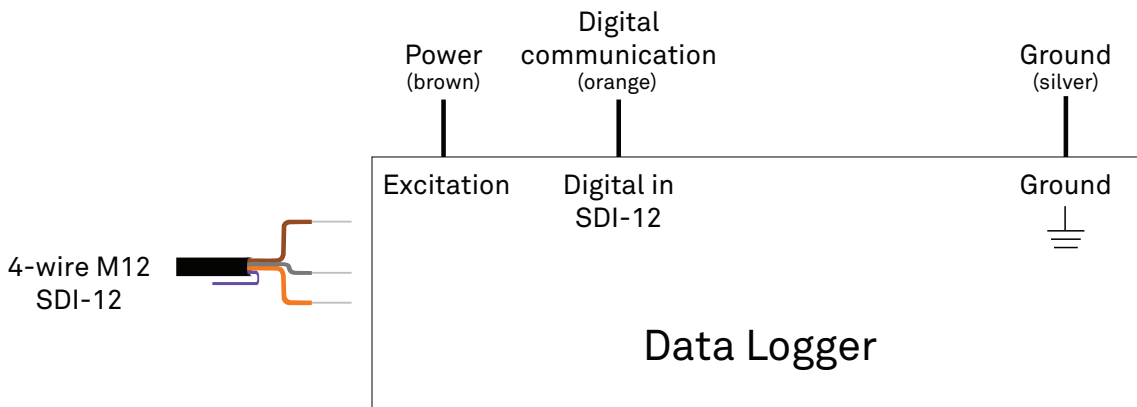
Figure 4 Four wire connector SDI-12 wiring diagram
