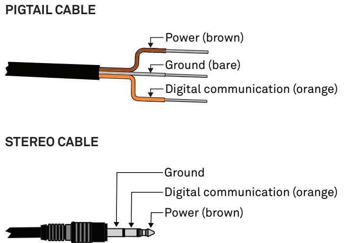
Figure 3 Connection types
