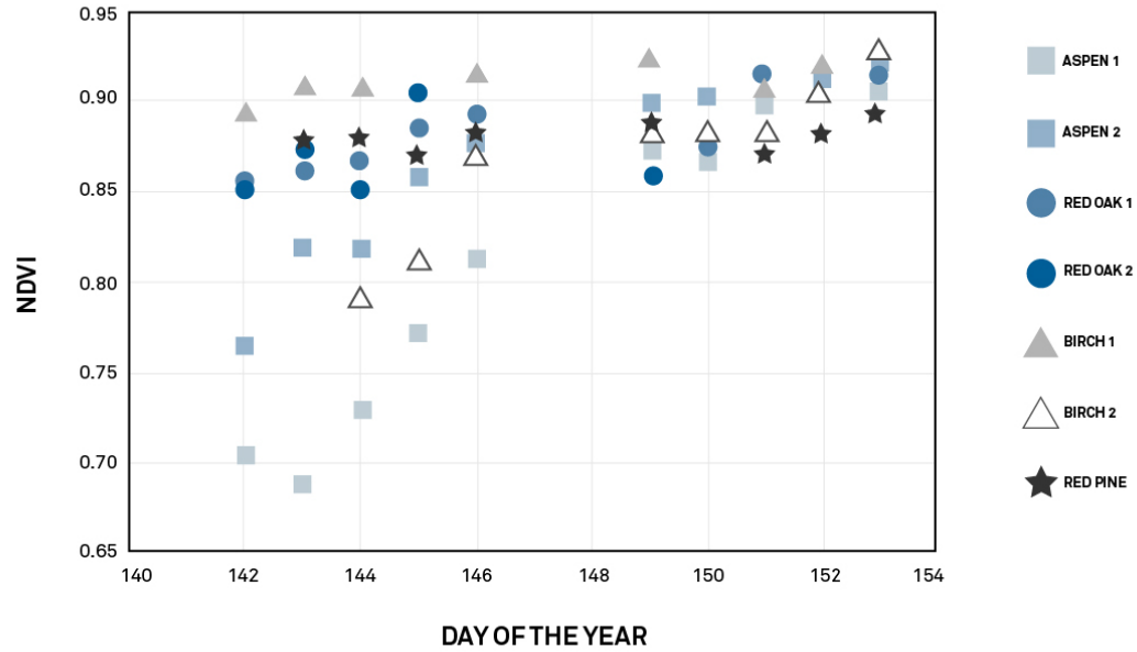
Figure 8 Spatial variability of NDVI during spring green up.
