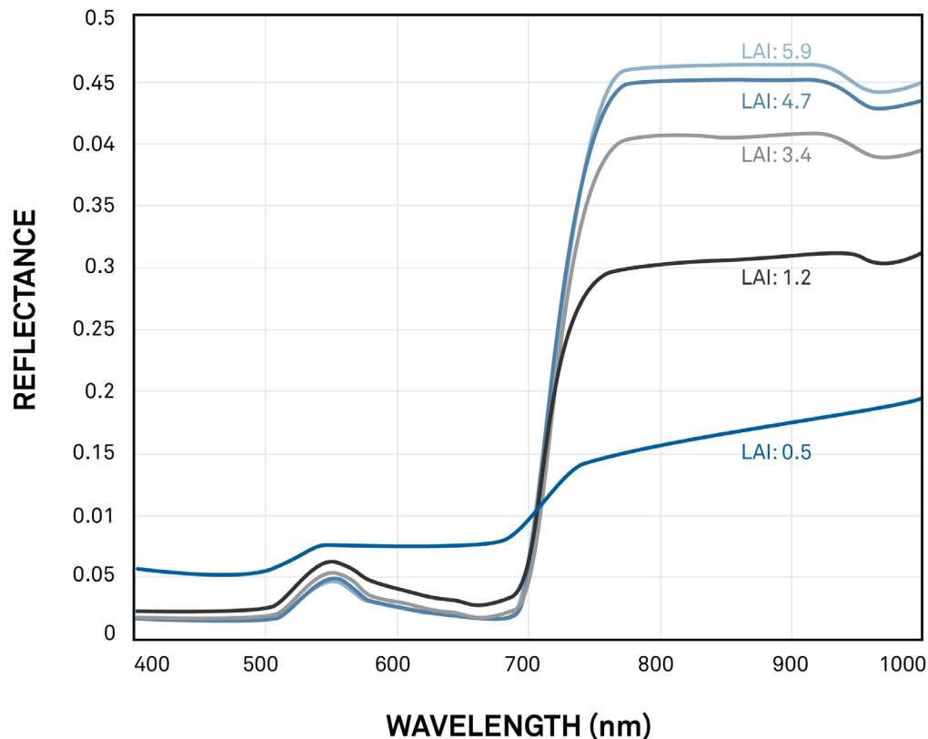
Figure 3 Reflectance spectra obtained at different stages of canopy development. Note: There is a distinct difference between visible and nearinfrared (NIR) reflectance that develops as LAI increases
