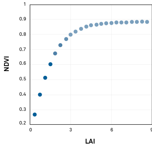
Figure 9 NDVI has limited sense to LAI values greater than 3-4
