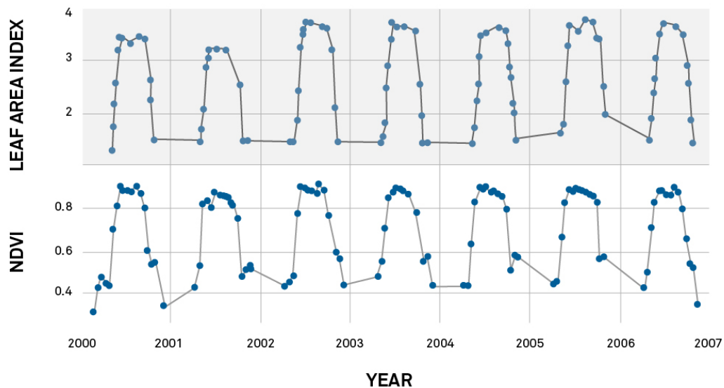
Figure 6 NDVI closely tracks the year to year seasonal dynamics of LAI in a mixed deciduous forest
