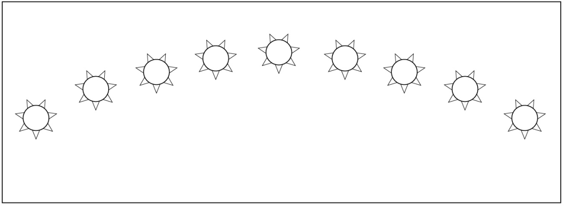
Figure 4 Solar zenith angle changes during the day. Observer is facing the equator
