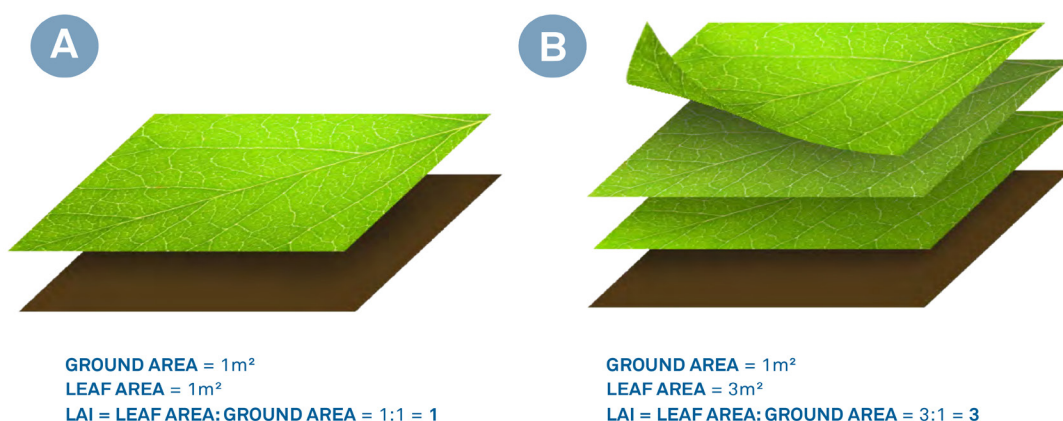
Figure 1 Conceptual diagram of a plant canopy where (a) LAI = 1 (b) LAI = 3
