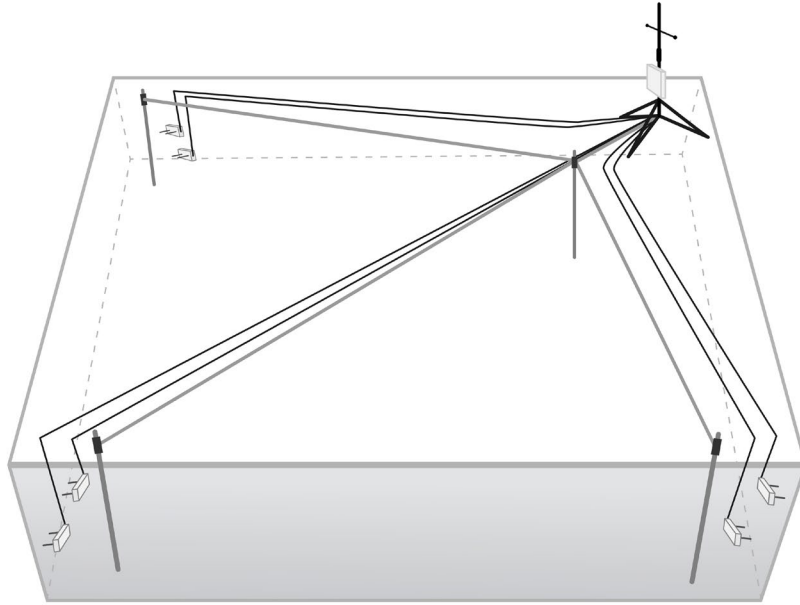
Figure 1. Ground rods in the general vicinity of groups of probes are connected back to a main grounding rod to which the logger is grounded. Ground rods should be driven at least 2 meters into the ground, if possible, and connected to the central ground through #6 AWG copper wire.
