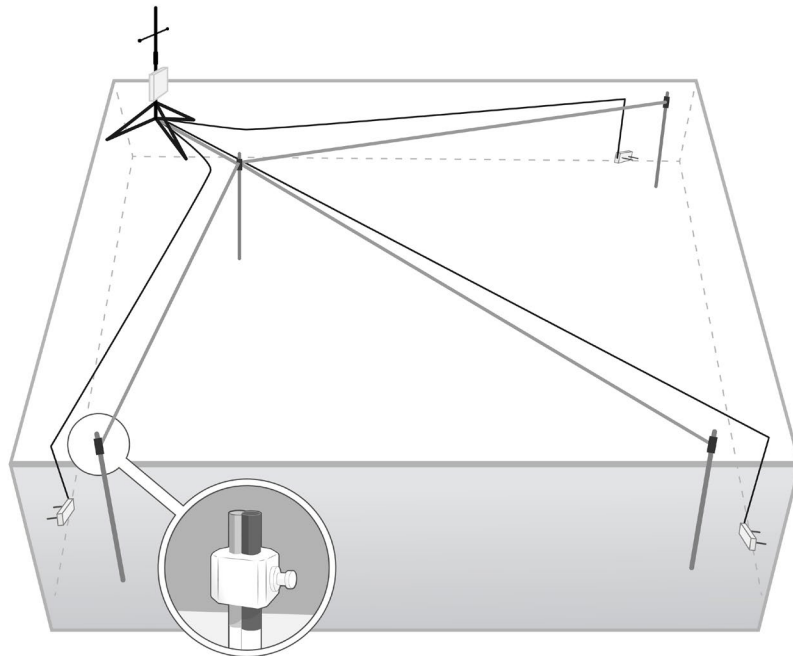
Figure 2. When lightning risk is high, ground rods may be required in the vicinity of each sensor location. As with the moderate lightning installation, #6 AWG copper wire connects each ground rod to the central rod, which is connected to the data logger
