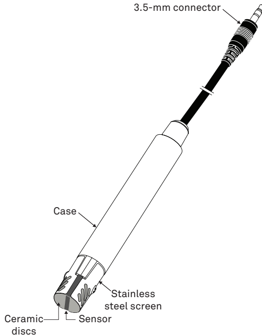
Figure 11 TEROS 22 sensor
