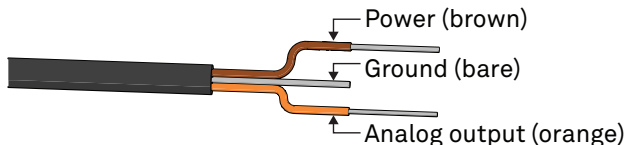
Figure 2 Pigtail wiring
