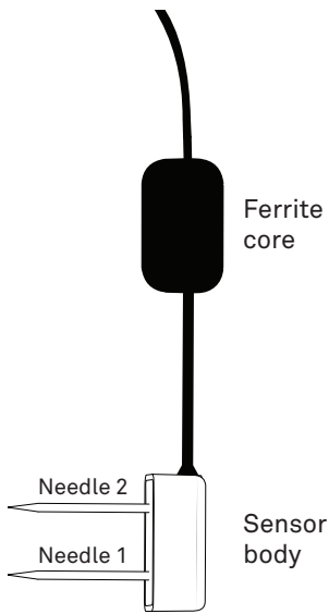
Figure 4 TEROS 10 sensor
