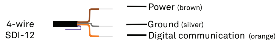
Figure 2 Pigtail wiring
