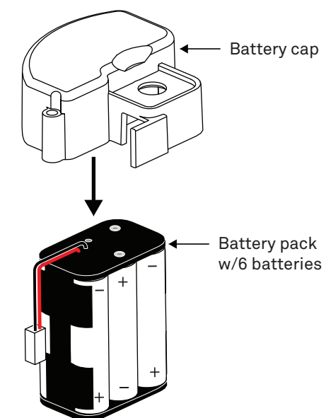
Figure 25 Battery pack removed from cap
