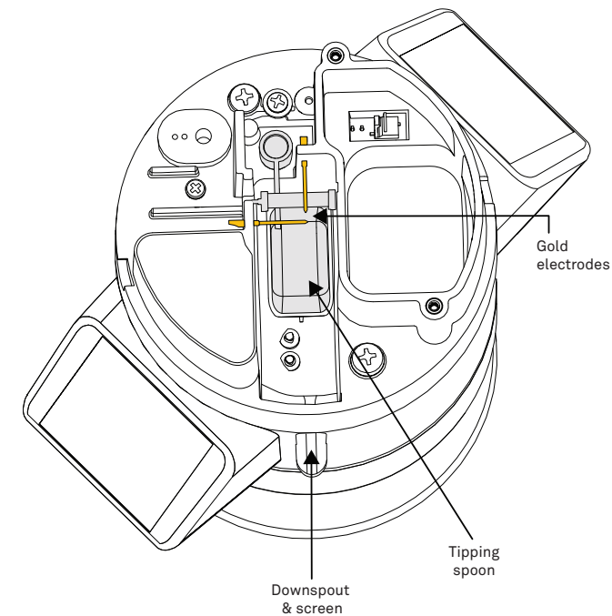
Figure 18 Downspout and screen
