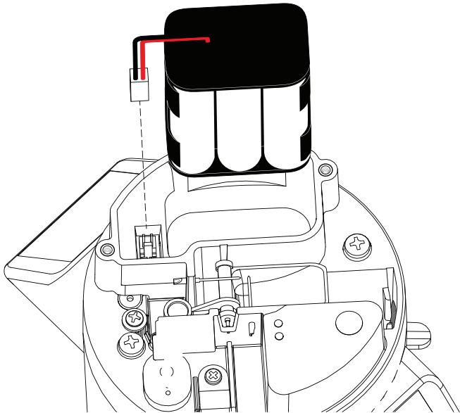
Figure 27 Battery pack with cable oriented for replacement
