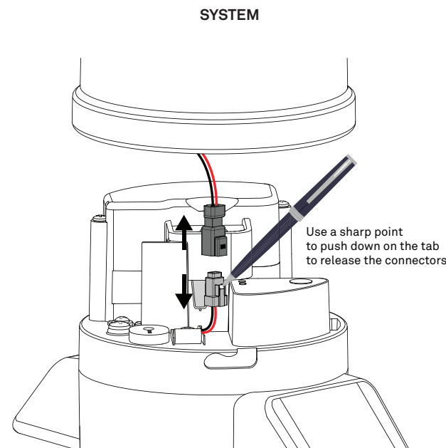
Figure 16 Disconnect pyranometer connector
