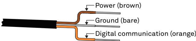
Figure 2 Pigtail wiring
