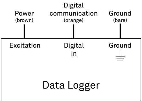
Figure 3 Wiring diagram
