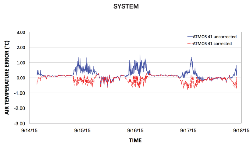
Figure 11 Corrected air temperature comparison with the aspirated radiation shield using 1-min measurement intervals
