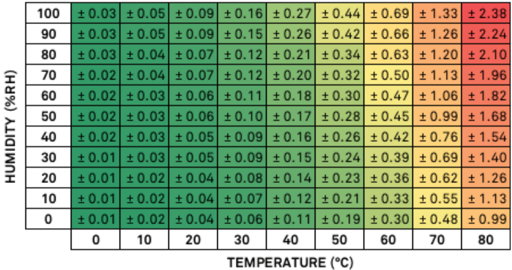
Figure 4 Vapor pressure sensor accuracy
