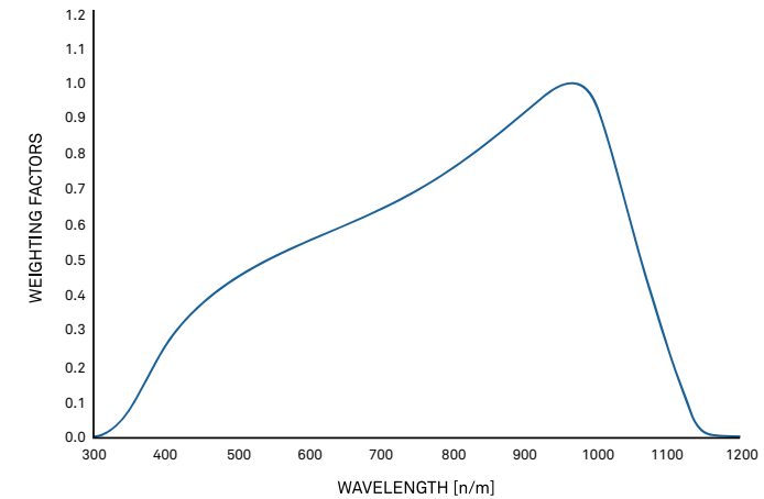
Figure 6 Spectral response estimate of Apogee silicon-cell pyranometers
