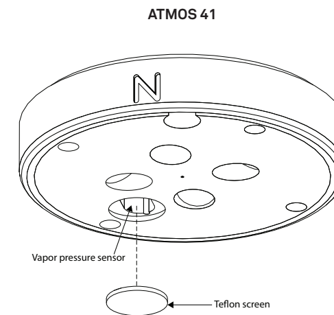
Figure 8 Vapor pressure sensor
