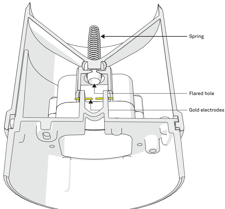
Figure 9 Rain gauge
