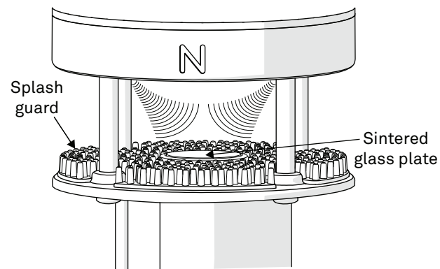
Figure 7 Anemometer
