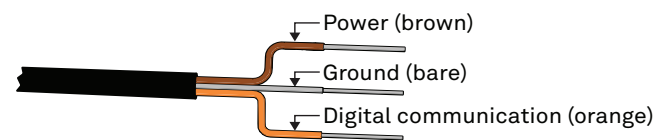
Figure 2 Pigtail wiring
