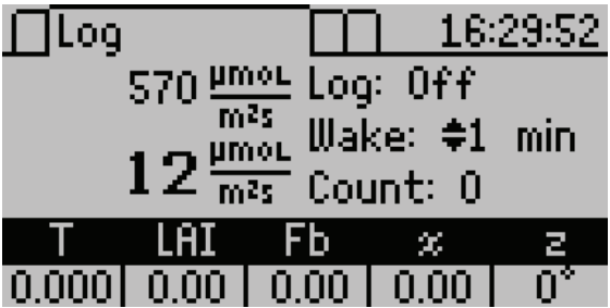
Figure 20 Log tab
