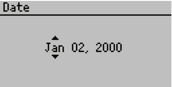
Figure 3 Date screen
