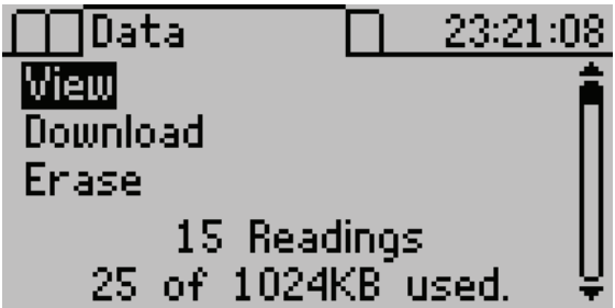
Figure 21 Data tab
