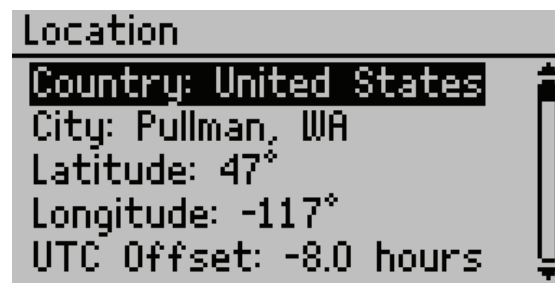
Figure 23 Location screen
