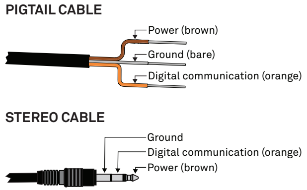
Figure 3 Connection types
