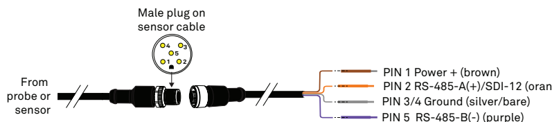
Figure 5 Four-wire M12 connector and pigtail adapter for use with screw terminals
