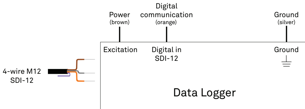
Figure 4 Four wire connector SDI-12 wiring diagram
